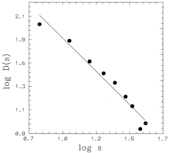
Fig. 1. Double logarithmic plot of the microtubule length distribution function D(s) at 14.4^\circ\text{C} for 45 \mu\text{m} tubulin concentration (data taken from Fygenso et al. , 1994). The straight line is a least-squares fit to the data. The \log s and \log D(s) denote decadic logarithms of s and D(s) , respectively. D(s) is the relative number of microtubules with the length s .
